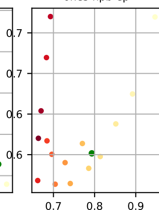
ones-npb-ep
