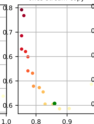
ones-stream-copy
