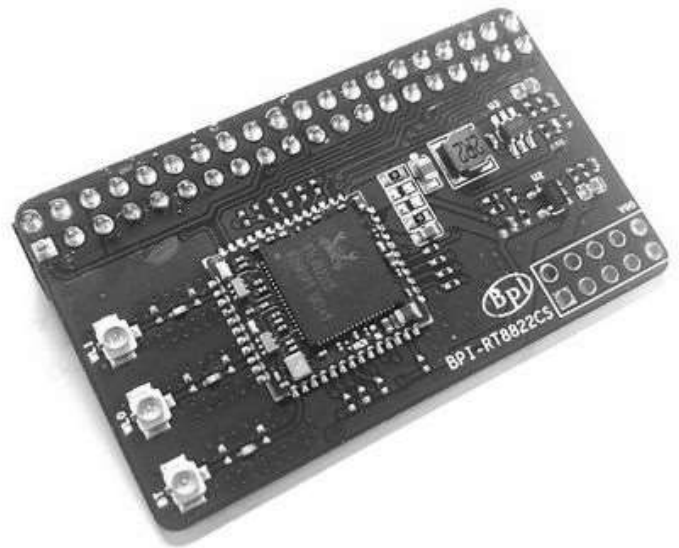
WiFi&BT board, 802.11 a/b/g/n/ac 2T2R WiFi and Bluetooth 5.0
