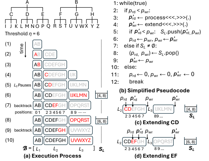
Figure 12: Example of Hybrid BFS-DFS Subgraph Extension
