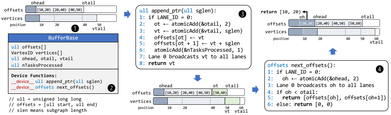
Figure 13: BufferBase and Its Operations
