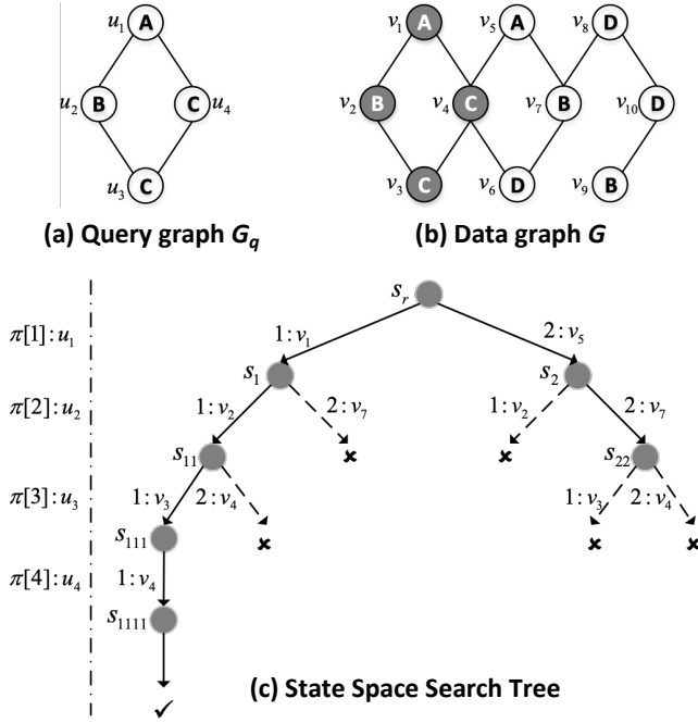
Figure 11: Illustration of Subgraph Matching
