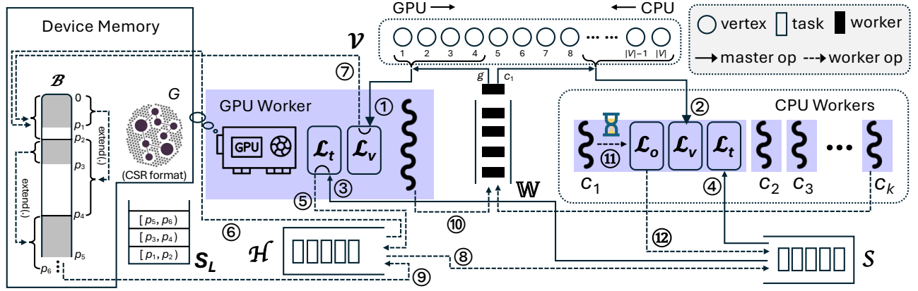
Figure 14: System Architecture and Task Flows in G-ThinkerCG
