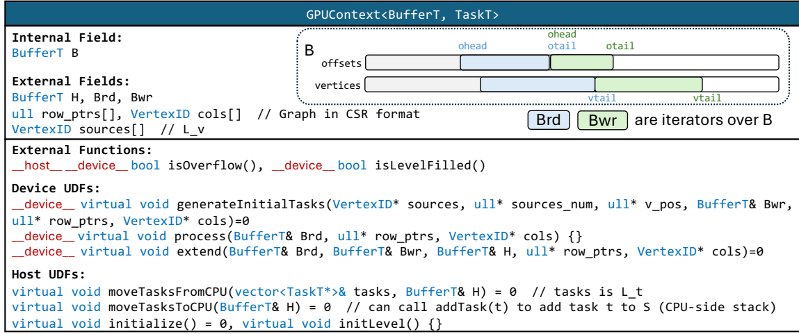
Figure 15: The GPUContext class with UDFs
