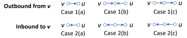
Fig. 9. Cases for Two-Hop Diameter Upper Bound
