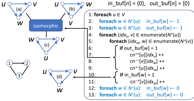
Fig. 8. Initial Counter Computation
