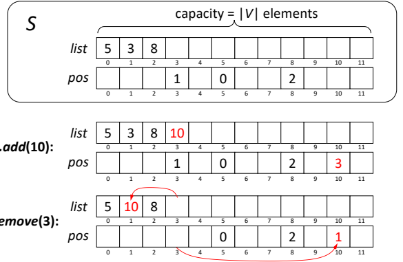
Fig. 10. Data Structure for Set Maintenance
