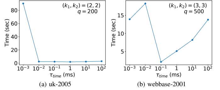
Fig. 11. Running Time When \tau_{time} is Varied
