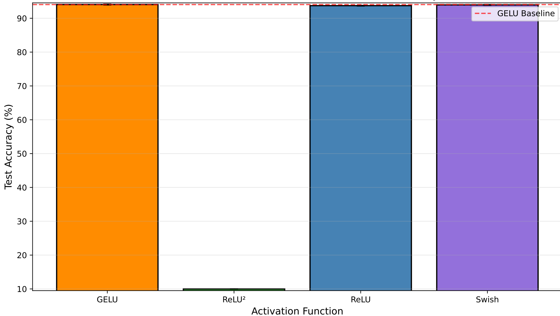
Effect of Activation Function on CIFAR-10 Accuracy
