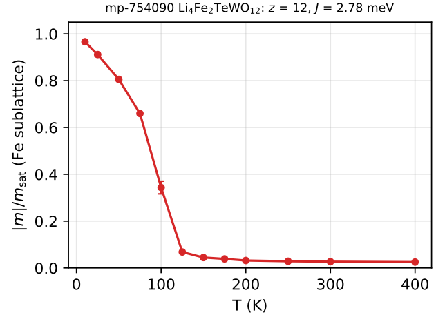
FIG. 6. Normalized net magnetization of the mp-754090 Fe sublattice (2048-spin cell) versus temperature, driven purely by the DFT-derived twelve-neighbor J = 2.78 meV with no fitting; 20 ps Langevin dynamics ( \alpha = 1 ), mean over three thermostat seeds (error bars: seed-to-seed standard deviation, smaller than the symbols except at 100 K). Runs start from the ordered state, so the absolute scale is physical ( |m| \rightarrow 1 as T \rightarrow 0 ); the high-temperature floor of \approx 0.025 is the 1/\sqrt{N} finite-size value of a 2048-spin paramagnet.
