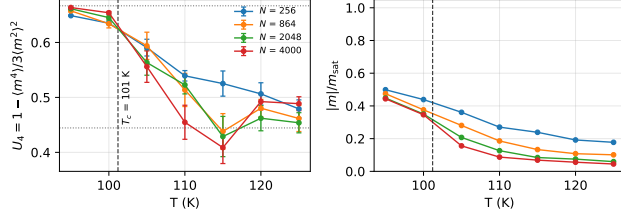
FIG. 7. Finite-size scaling of the mp-754090 spin model. Left: Binder cumulant U_4 = 1 - \langle m^4 \rangle / 3 \langle m^2 \rangle^2 at four system sizes with the box aspect ratio held fixed ( N = 256, 864, 2048 and 4000 spins), from 40 ps Langevin dynamics ( \alpha = 1 ) with the moments pooled over the last 20 ps of four thermostat seeds; error bars are a drop-one-seed jackknife. Dotted lines mark the ordered ( 2/3 ) and disordered ( 4/9 ) limits of a three-component order parameter and the dashed line the mean of the three pairwise crossings, T_c = 101 K. Right: |m|(T) at the same four sizes, showing the collapse sharpening with N .
