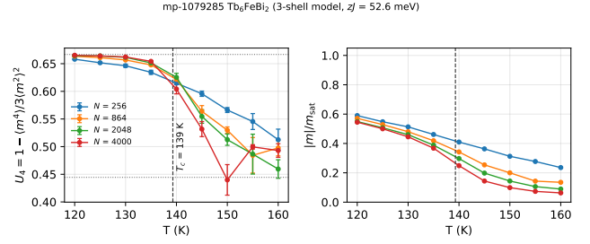
FIG. 9. Finite-size scaling of the mp-1079285 three-shell model, as Fig. 7: Binder cumulant (left) and |m| (right) at N = 256, 864, 2048 and 4000 spins with the box aspect ratio held fixed. Four 40 ps seeds per point at 120–130 and 155–160 K; 10–14 seeds at 135–150 K, where the crossings lie, six of them 80 ps. The dashed line is the mean of the three pairwise crossings, T_c = 139 K.
