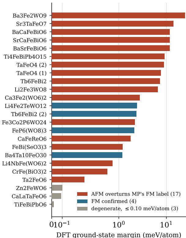
DFT-validated ordering vs. MP's stored FM label (24 DMI-shortlisted candidates)
