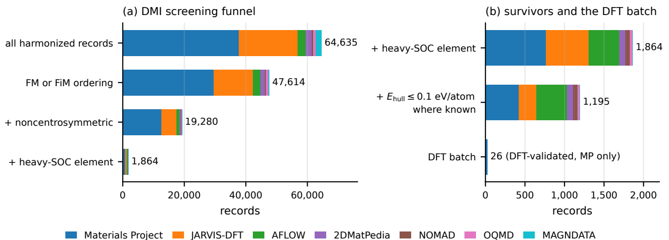
FIG. 2. The DMI-compatibility screening funnel by source database. (a) Each successive criterion – net-moment ordering (ground-truth label where present, otherwise the deployed classifier’s prediction), noncentrosymmetric space group, and at least one heavy spin-orbit-coupling element – applied to the 64,635-record harmonized database. (b) The 1,864 survivors, the 1,195 that remain when a known hull distance above 0.1 eV/atom is used as a hard exclusion (sources without a hull field are retained), and the 26-candidate DFT batch, which is Materials Project only.
