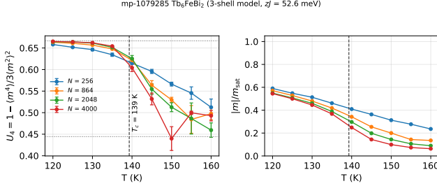
FIG. 9. Finite-size scaling of the mp-1079285 three-shell model, as Fig. 7: Binder cumulant (left) and |m| (right) at N = 256, 864, 2048 and 4000 spins with the box aspect ratio held fixed. Four 40 ps seeds per point at 120–130 and 155–160 K; 10–14 seeds at 135–150 K, where the crossings lie, six of them 80 ps. The dashed line is the mean of the three pairwise crossings, T_c = 139 K.
