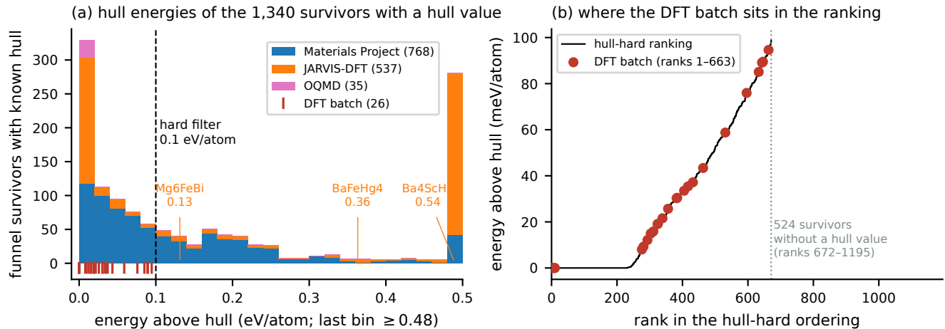
FIG. 3. Thermodynamic stability of the funnel survivors. (a) Distribution of the hull distance for the 1,340 survivors that carry one (Materials Project and OQMD as stored; JARVIS recomputed from its own formation energies, see text), with the 0.1 eV/atom hard filter and the three JARVIS entries of the original top-30 shortlist that it removes; red ticks mark the 26 DFT-batch candidates. (b) Hull distance versus rank in the hard-filtered ordering, which sorts stable records by hull distance first: the DFT batch (red) spans ranks 1–663, so it is a sample of the funnel’s DMI-compatible population, not of its most stable members.
