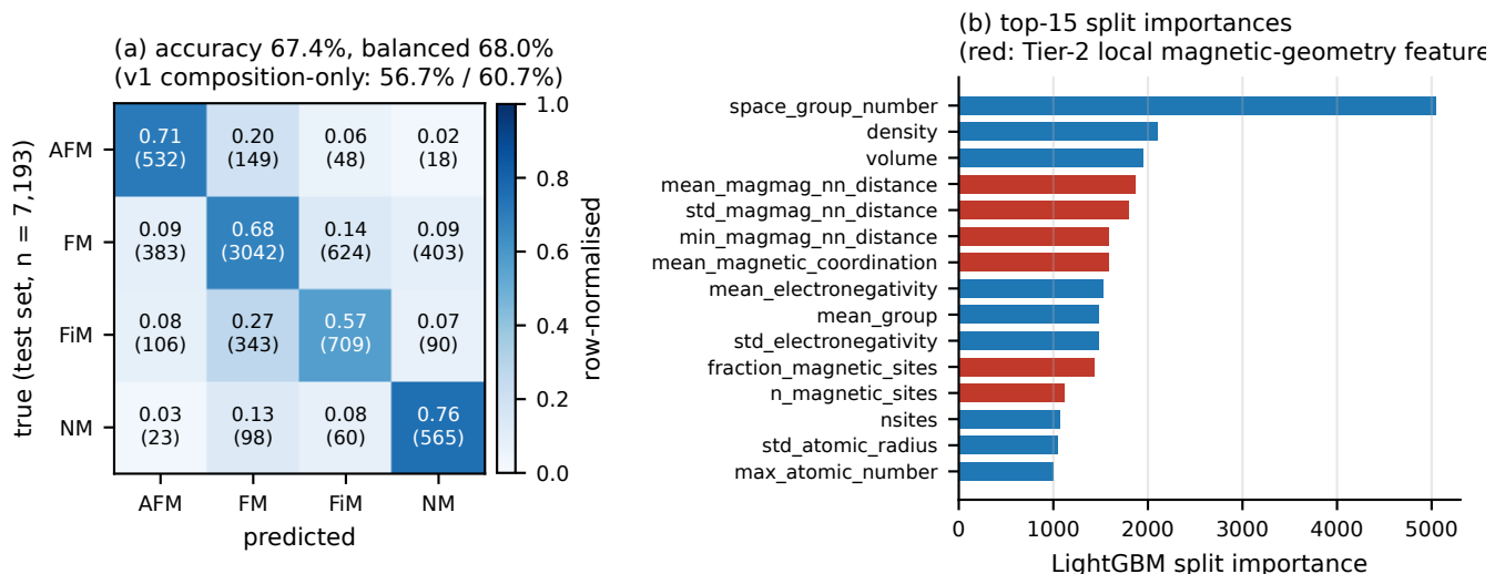
FIG. 1. Structure-aware ordering classifier on the held-out test set (7,193 records, stratified 80/20 split). (a) Row-normalised confusion matrix (counts in parentheses): the dominant confusion is FM \rightarrow FiM and FiM \rightarrow FM, i.e. between the two net-moment classes that the screening funnel treats identically, whereas AFM and NM are recovered at 71% and 76%. (b) The fifteen most-used features by LightGBM split count; the six Tier-2 local-magnetic-geometry features (red), computed from atomic positions and species only, now sit alongside the space-group and density/volume descriptors instead of acting as a MAGNDATA source flag.
