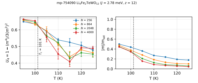
FIG. 7. Finite-size scaling of the mp-754090 spin model. Left: Binder cumulant U_4 = 1 - \langle m^4 \rangle / 3 \langle m^2 \rangle^2 at four system sizes with the box aspect ratio held fixed ( N = 256, 864, 2048 and 4000 spins), from 40 ps Langevin dynamics ( \alpha = 1 ) with the moments pooled over the last 20 ps of four thermostat seeds; error bars are a drop-one-seed jackknife. Dotted lines mark the ordered ( 2/3 ) and disordered ( 4/9 ) limits of a three-component order parameter and the dashed line the mean of the three pairwise crossings, T_c = 101 K. Right: |m|(T) at the same four sizes, showing the collapse sharpening with N .
