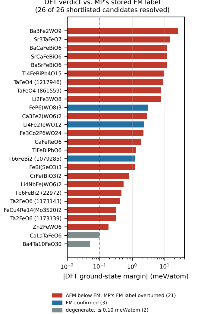
FIG. 4. DFT ground-state margin for the 26 candidates, sorted by magnitude (logarithmic horizontal axis; only calculations that converged and passed the spin-state audit enter, and a tight same-cell pair replaces the loose number whenever one exists). Twenty-one candidates’ MP-recorded FM label is overturned by a lower-energy AFM or FiM configuration (red); three are confirmed as the true FM ground state (blue); two sit at or below the electronic-convergence tolerance ( \leq 0.10 meV/atom, gray) and are read as degenerate rather than informative. Duplicate formulas are distinguished by their MP identifier.
