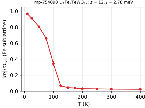
FIG. 6. Normalized net magnetization of the mp-754090 Fe sublattice (2048-spin cell) versus temperature, driven purely by the DFT-derived twelve-neighbor J = 2.78 meV with no fitting; 20 ps Langevin dynamics ( \alpha = 1 ), mean over three thermostat seeds (error bars: seed-to-seed standard deviation, smaller than the symbols except at 100 K). Runs start from the ordered state, so the absolute scale is physical ( |m| \rightarrow 1 as T \rightarrow 0 ); the high-temperature floor of \approx 0.025 is the 1/\sqrt{N} finite-size value of a 2048-spin paramagnet.
