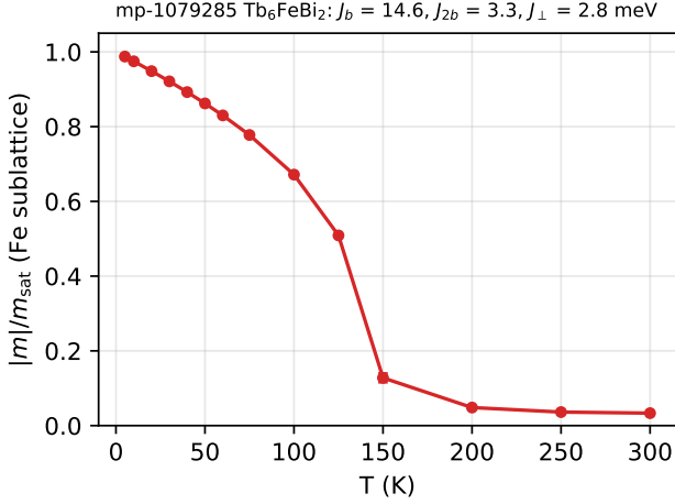
FIG. 8. Normalized net magnetization of the mp-1079285 Fe sublattice (2048-spin cell) versus temperature from the three-shell model with DFT-derived J_b = 14.61 , J_{2b} = 3.31 , J_\perp = 2.80 and |\mathbf{D}| = 0.098 meV; 20 ps Langevin dynamics ( \alpha = 1 ) from the ordered state, mean over three thermostat seeds (error bars: seed-to-seed standard deviation, smaller than the symbols except at 150 K).
