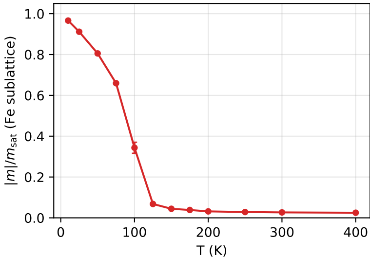
mp-754090 \text{Li}_4\text{Fe}_2\text{TeWO}_{12} : z = 12 , J = 2.78 meV
