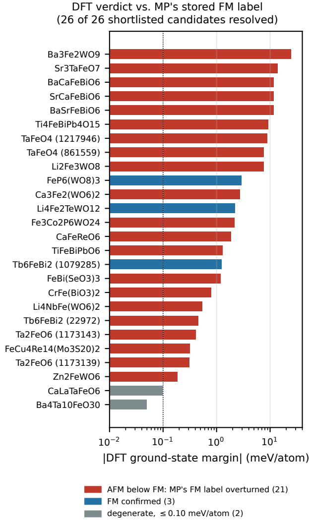
FIG. 4. DFT ground-state margin for the 26 candidates, sorted by magnitude (logarithmic horizontal axis; only calculations that converged and passed the spin-state audit enter, and a tight same-cell pair replaces the loose number whenever one exists). Twenty-one candidates' MP-recorded FM label is overturned by a lower-energy AFM or FiM configuration (red); three are confirmed as the true FM ground state (blue); two sit at or below the electronic-convergence tolerance ( \leq 0.10 meV/atom, gray) and are read as degenerate rather than informative. Duplicate formulas are distinguished by their MP identifier.
