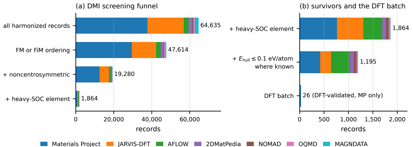
FIG. 2. The DMI-compatibility screening funnel by source database. (a) Each successive criterion – net-moment ordering (ground-truth label where present, otherwise the deployed classifier’s prediction), noncentrosymmetric space group, and at least one heavy spin-orbit-coupling element – applied to the 64,635-record harmonized database. (b) The 1,864 survivors, the 1,195 that remain when a known hull distance above 0.1 eV/atom is used as a hard exclusion (sources without a hull field are retained), and the 26-candidate DFT batch, which is Materials Project only.
