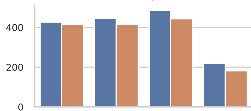
MobileNetV2 | 2 threads
