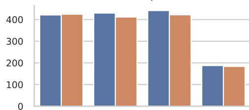
MobileNetV2 | 4 threads
