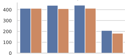
MobileNetV2 | 1 thread
