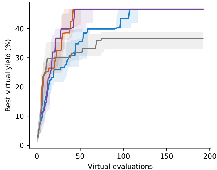
onehot GP
