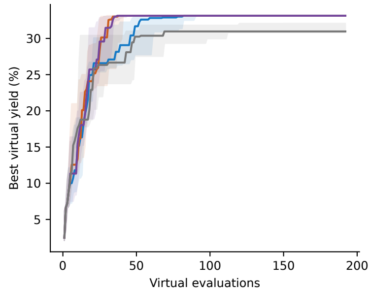
onehot RF
