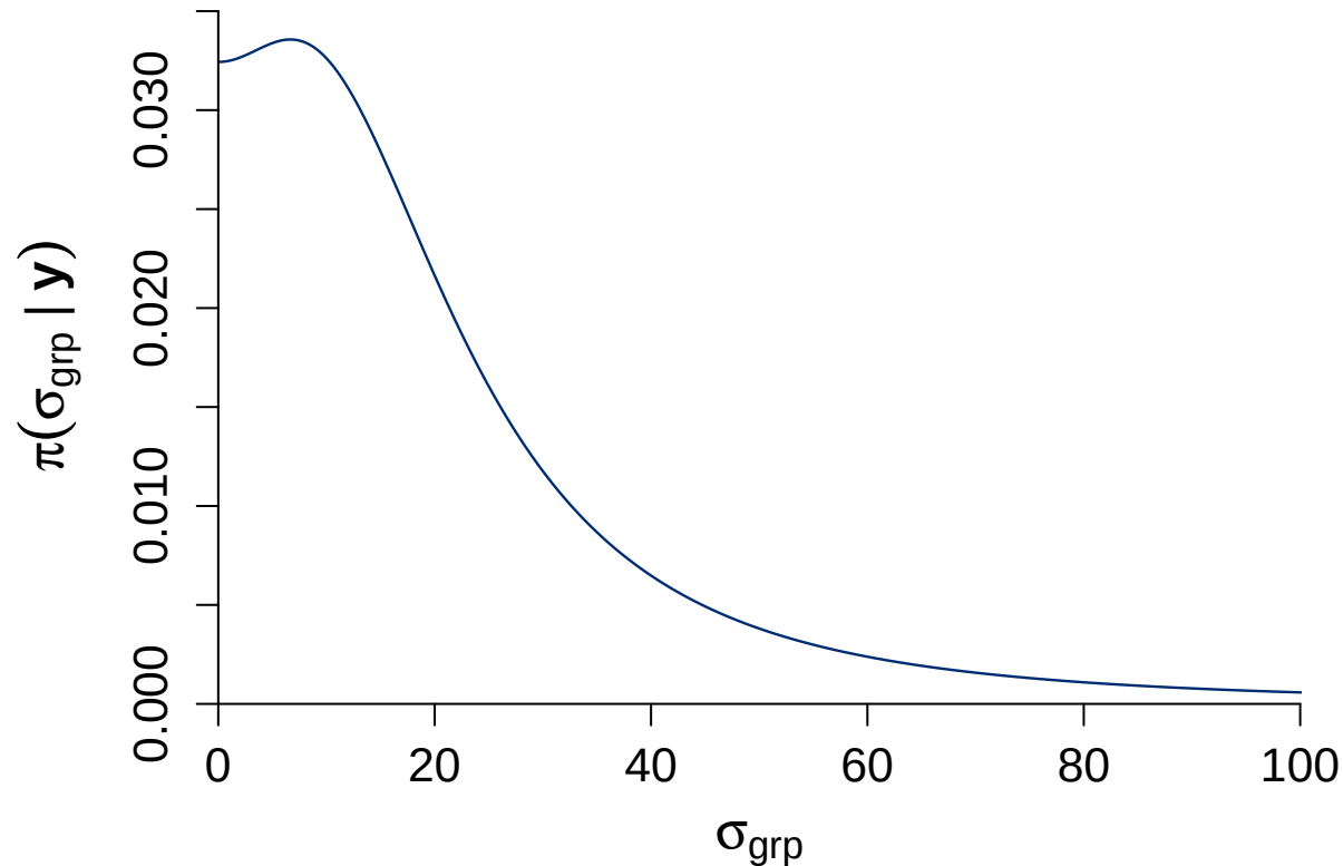
Posterior with 3 schools
