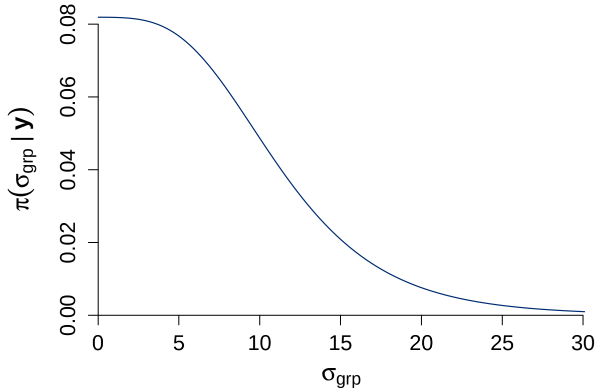
Posterior with 8 schools
