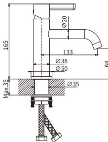
Cartridge: 25 mm Spout height: 68mm Projection: 133 mm
