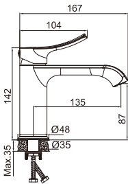
Cartridge: 35 mm Spout height: 87 mm Projection: 135 mm
