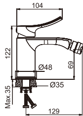
Cartridge: 35 mm Spout height: 69 mm Projection: 129 mm
