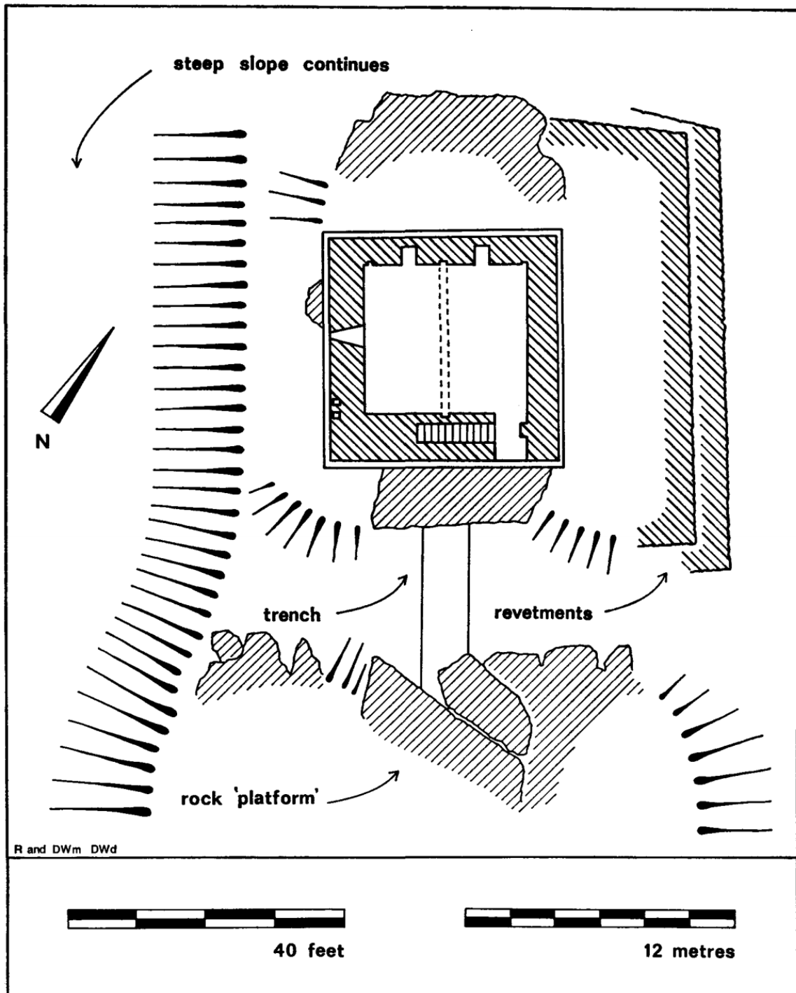
FIG. 5.—SITE A1. NOTE, THE TOWER IS PLANNED AT FIRST FLOOR LEVEL
