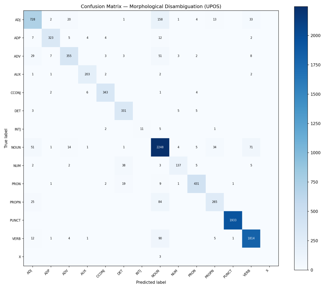
Figure 2. Confusion matrix on the treebank test set. Diagonal = correct predictions. Rows = true label, Columns = predicted label.
