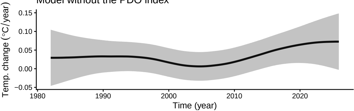
Model without the PDO index
