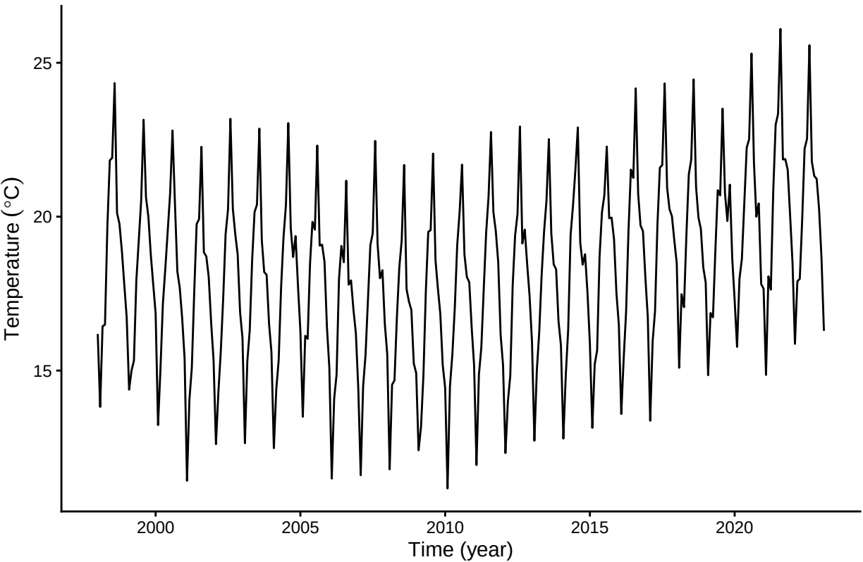
Simulated monthly SST off Jogashima, Japan
