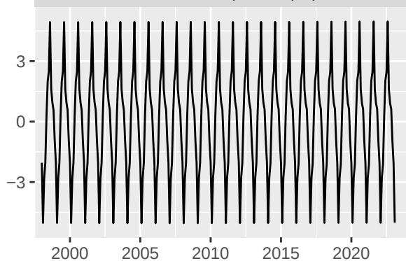
Seasonal component ( ^{\circ}\text{C} )
