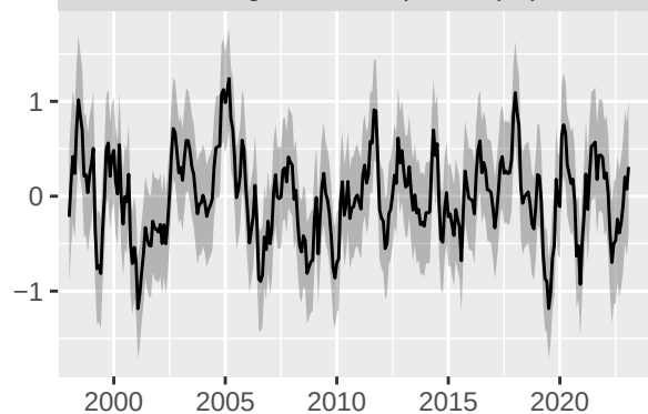
Autoregressive component ( ^{\circ}\text{C} )
