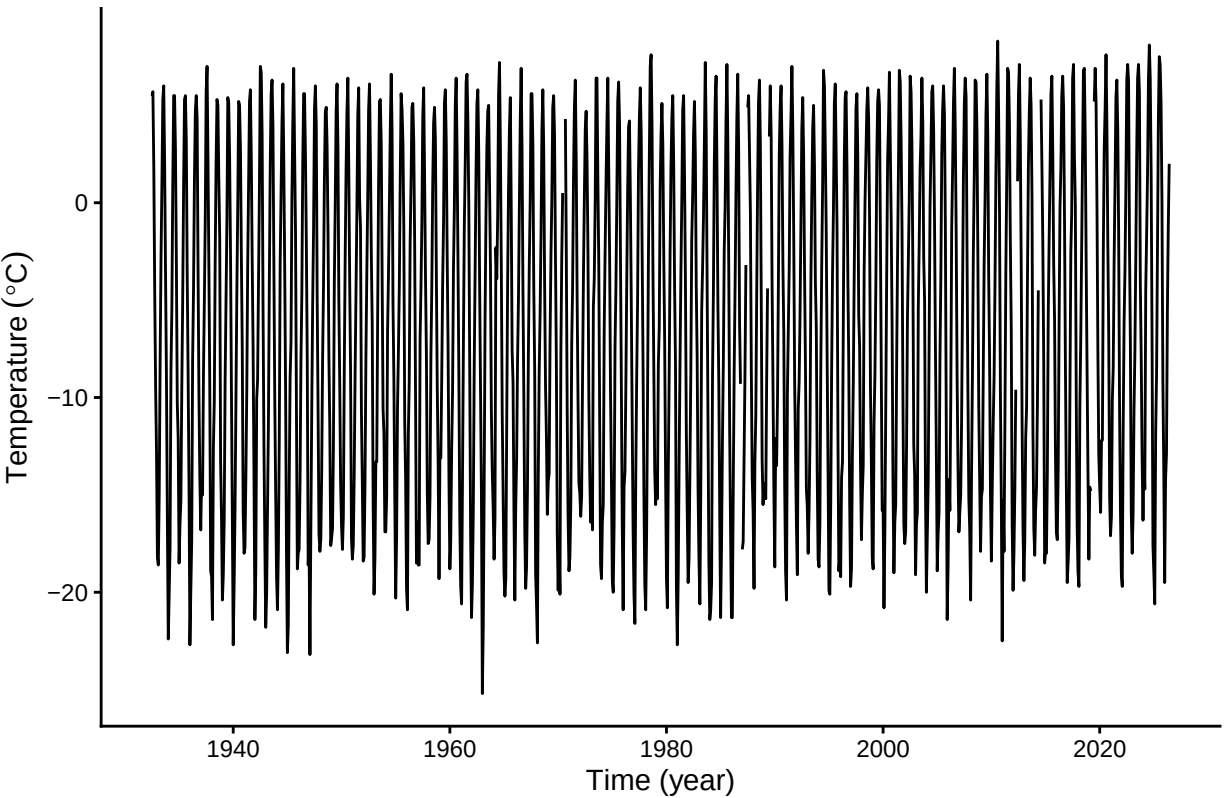
Monthly air temperature at the summit of Mt. Fuji
