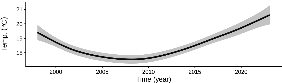
Model with Kuroshio variables
