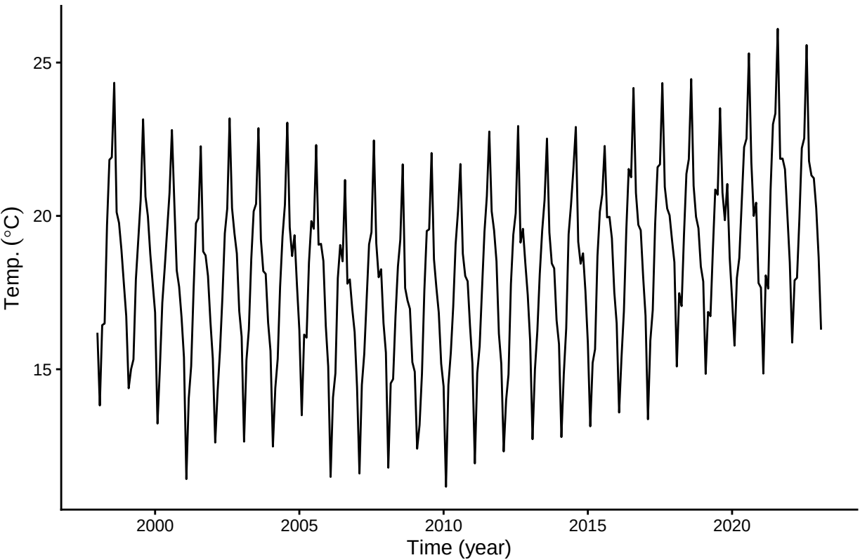
Monthly SST off Jogashima, Japan
