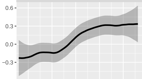
Drift component ( ^{\circ}\text{C}/\text{year} )
