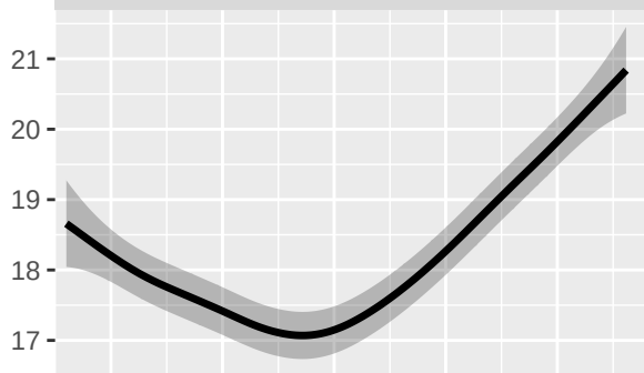
Level component ( ^{\circ}\text{C} )
