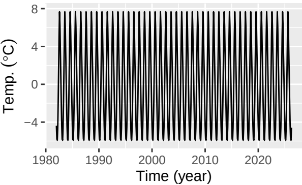
Seasonal component
