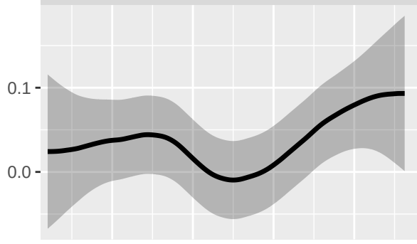
Autoregressive (1) component ( ^{\circ}\text{C} )
