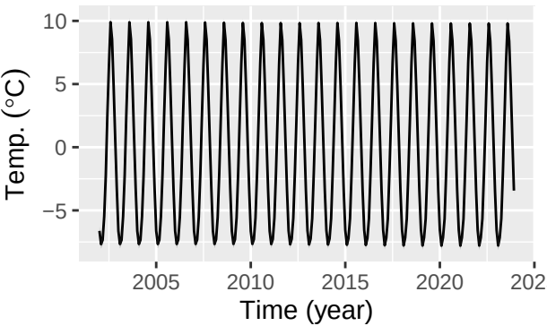
Seasonal component
