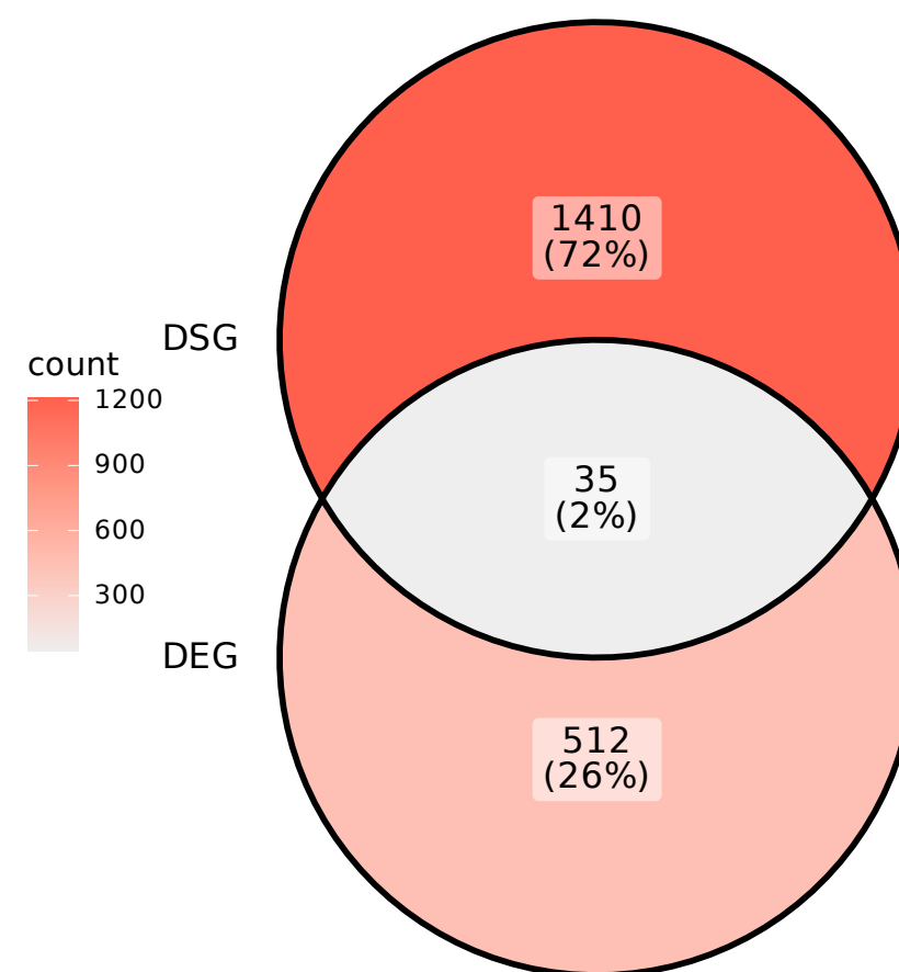
Tra2b
