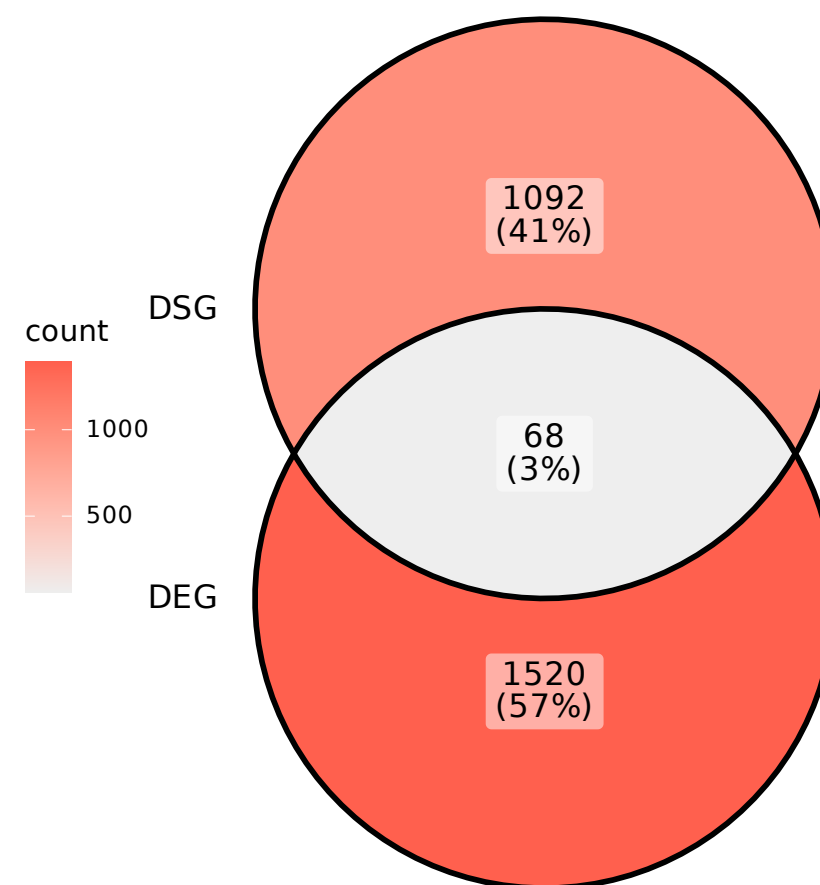
Ybx1
