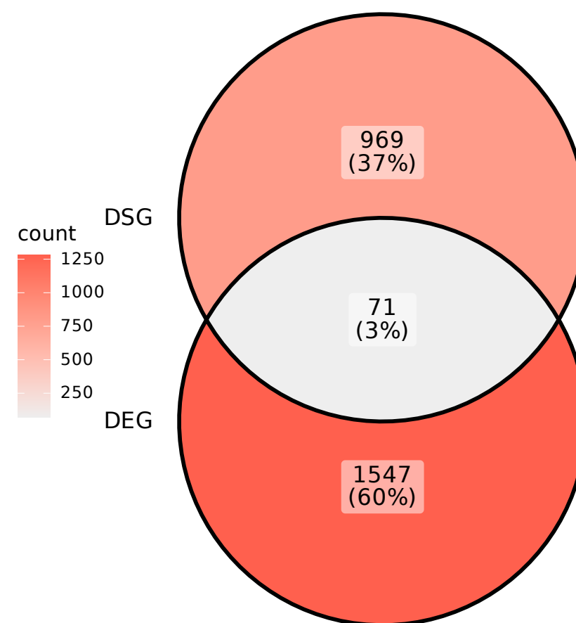
Ybx1
