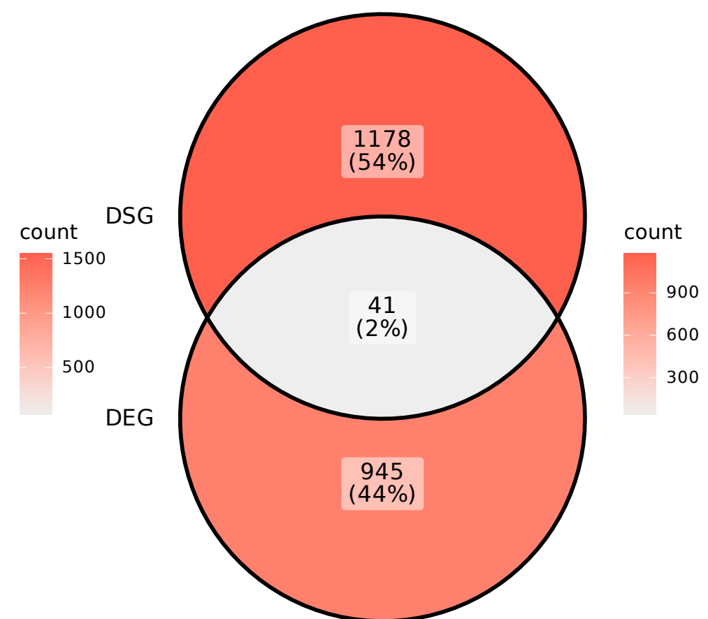
Trim71
