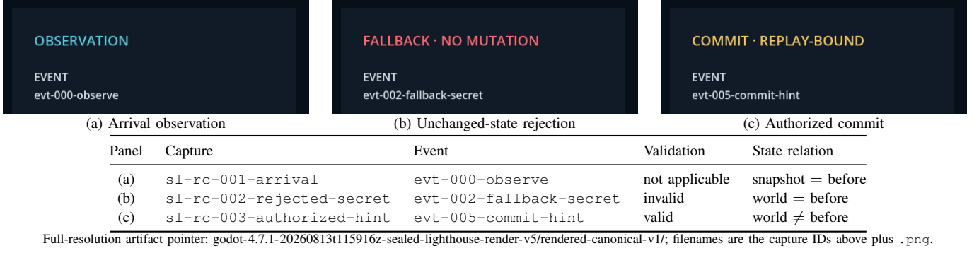
Fig. 4. Illustrative status/event crops from the authored Godot render replay, with manifest metadata. The trace-bound correspondence is not live-transport, performance, usability, immersion, or efficacy evidence.
