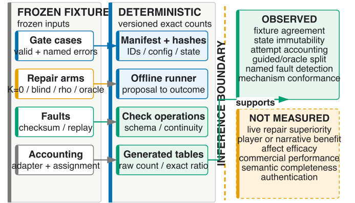
Fig. 5. Evidence boundary from frozen fixture through a designated check operation and generated table. Counts are admitted only through generated artifacts.
