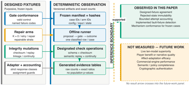
Fig. 4. Evidence boundary from frozen fixture through a designated check operation and generated table. Counts are admitted only through generated artifacts.
