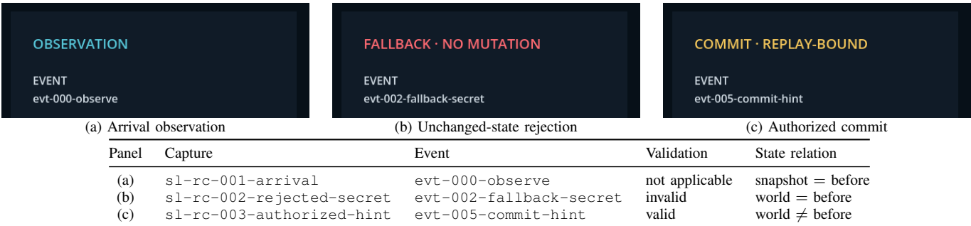
Fig. 5. Illustrative status/event crops from the authored Godot render replay, with manifest metadata. The trace-bound correspondence is not live-transport, performance, usability, immersion, or efficacy evidence.
