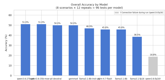
Figure 3: Overall accuracy by model across all eight scenarios and twelve repeats
