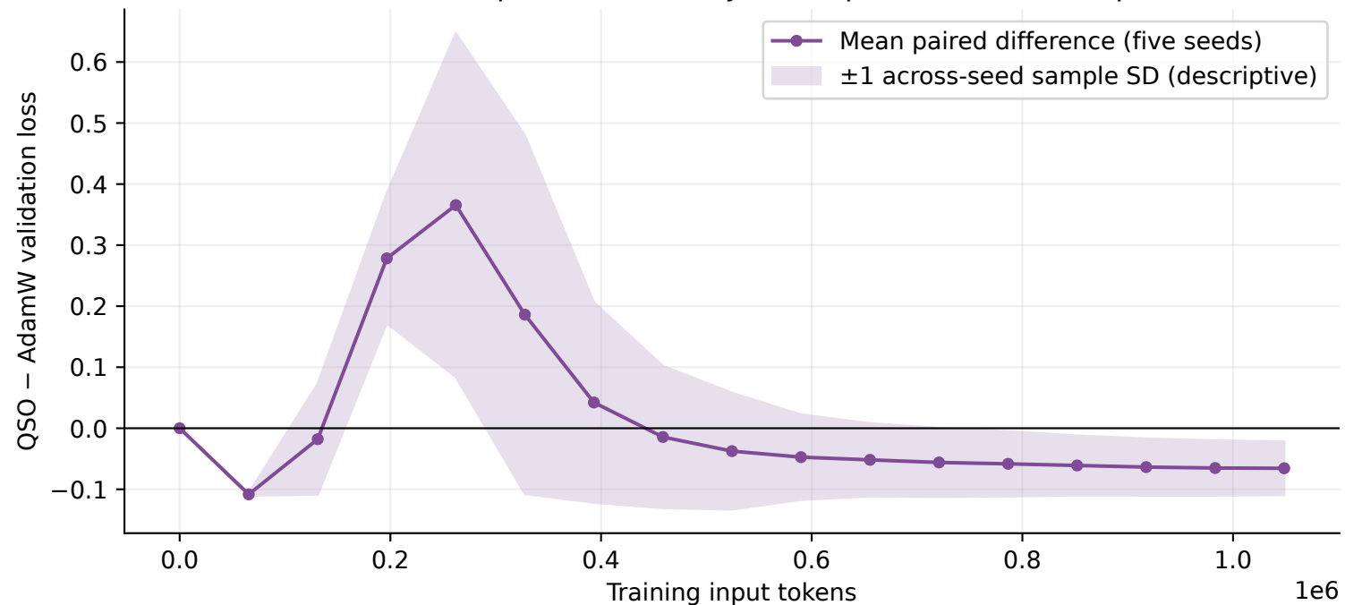
Across-seed descriptive uncertainty; checkpoints are not independent
