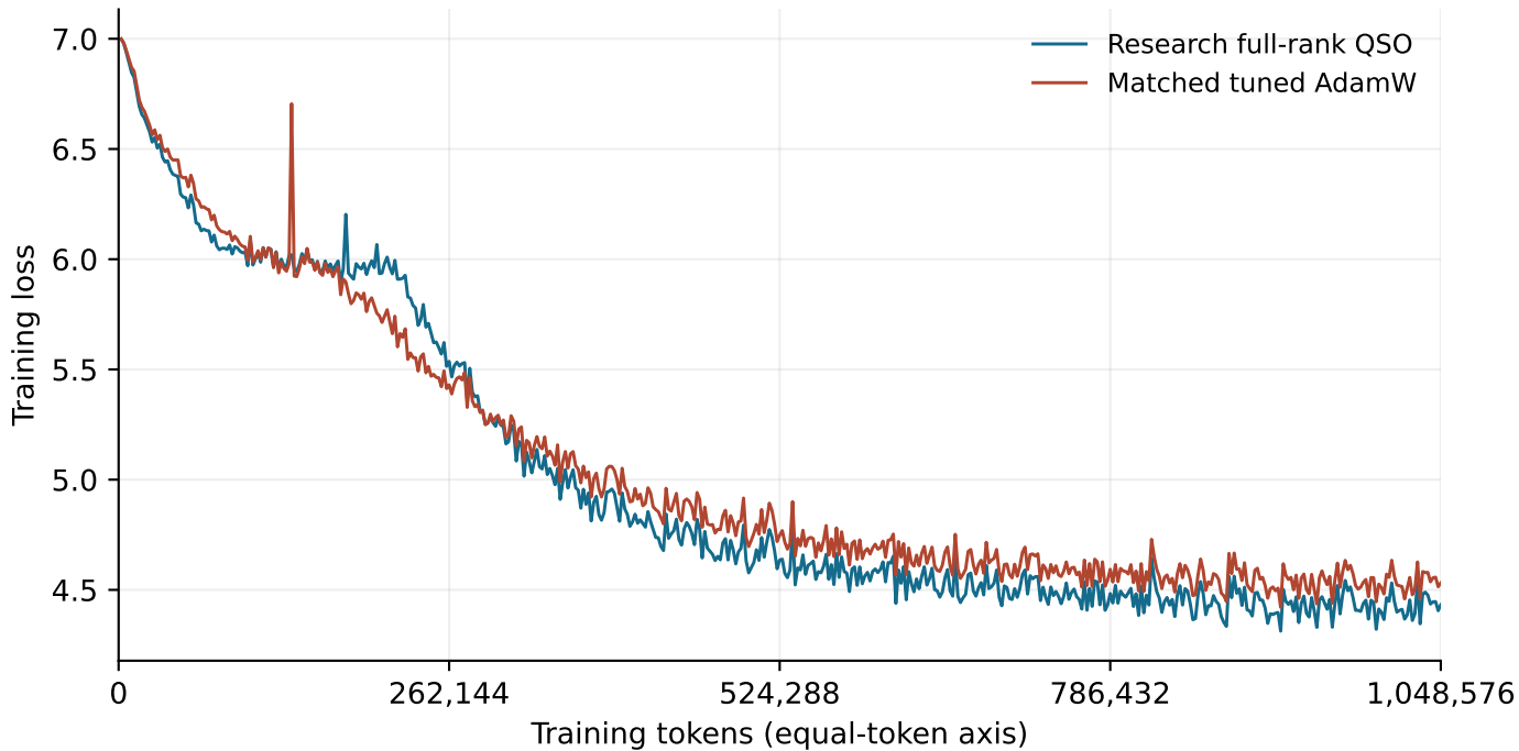
Recorded training losses (unsmoothed)
