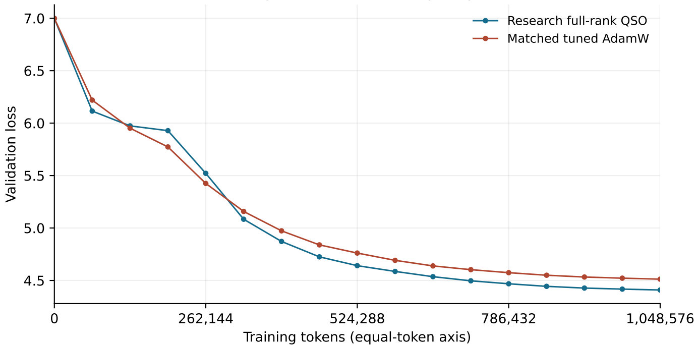
Single-seed validation quality
