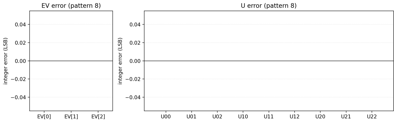
Figure 5.1: RTL vs. bit-true model error (pattern 8).
