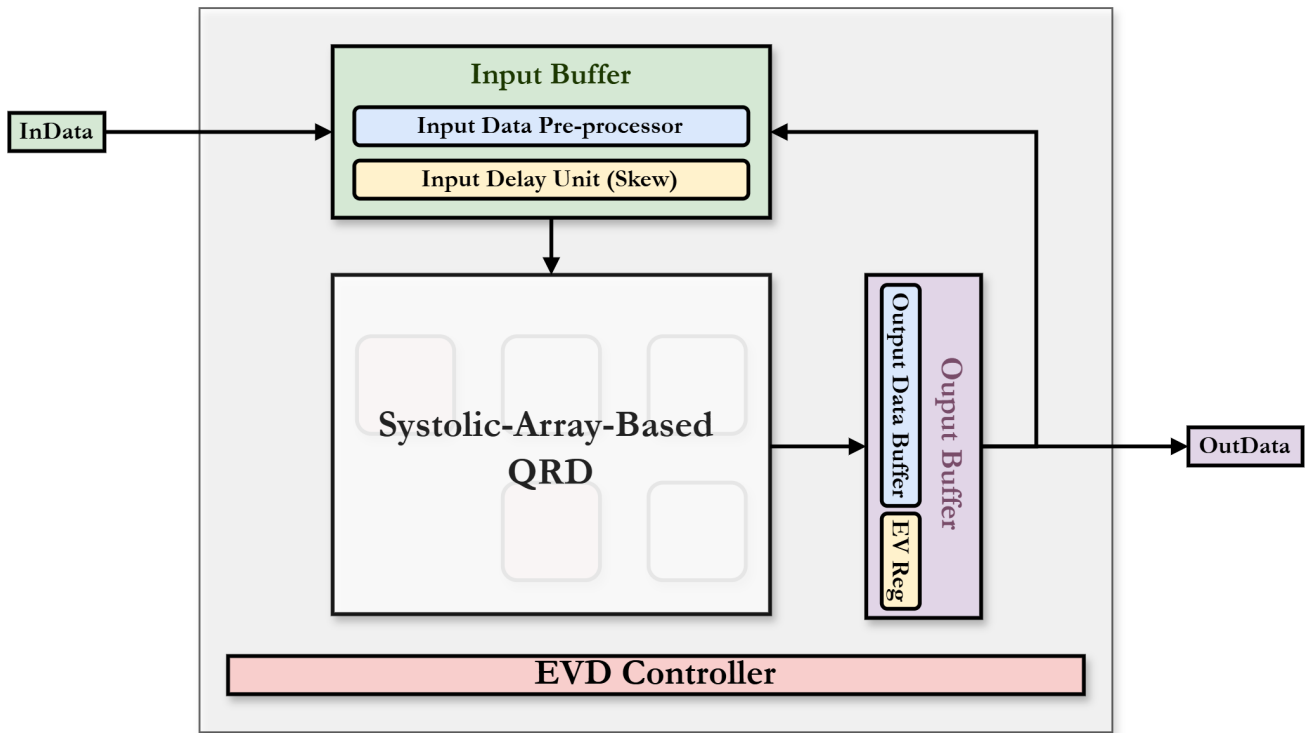
Figure 3.4: Top-level EVD architecture.
