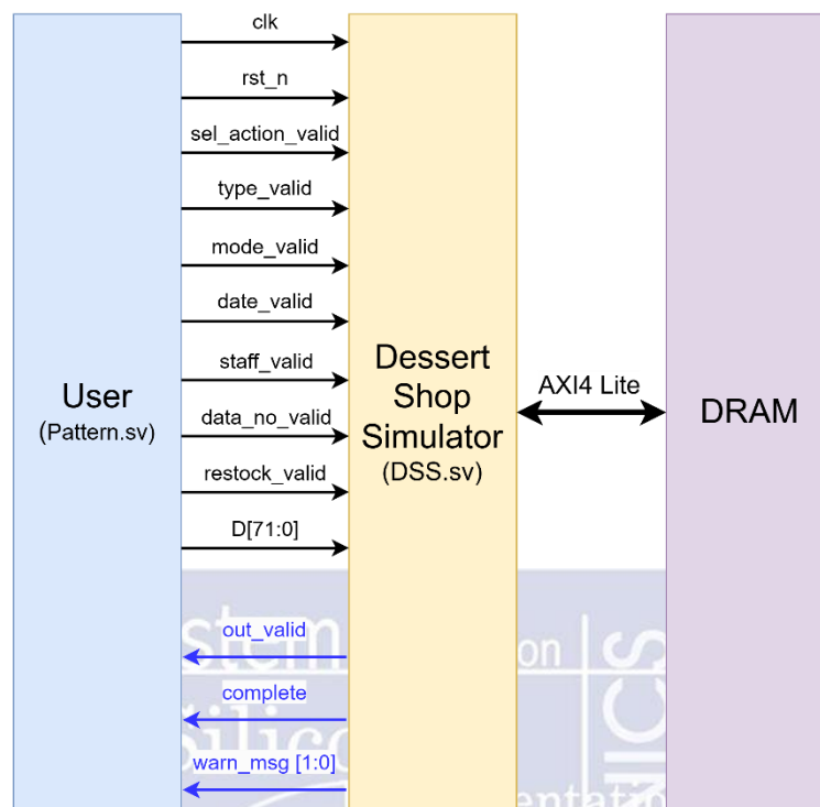
Figure 1: The Design Block Diagram
