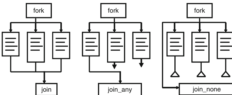
Fig. 7.2 Fork...join blocks
