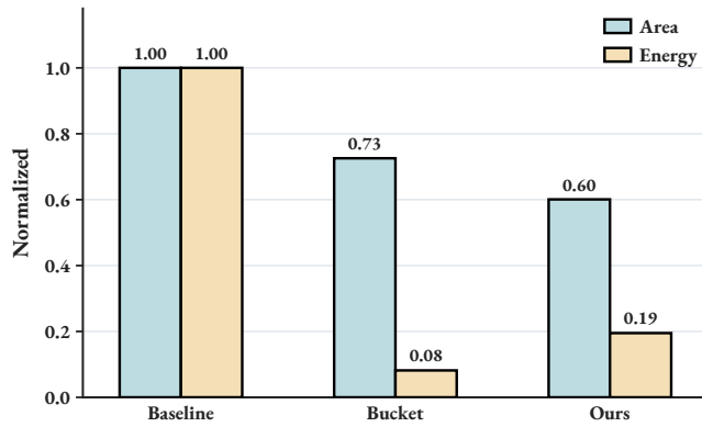
Figure 9: Normalized PE area and energy of a BFP4 baseline, a Bucket Getter PE, and the proposed PE (TSMC 90 nm, 125 MHz). Both metrics are normalized to the baseline.
