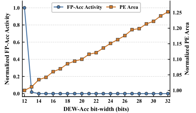
Figure 8: Normalized FP-Acc overflow activity and synthesized PE area versus DEW-Acc bit-width on LLaMA2-7B (W-BFP4 / T2A-BiE4, G16, (T_{\text{drop}}, T_{\text{replace}}) = (9, 3) ). Both series are normalized to W12.
