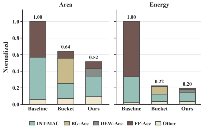
Figure 9: Normalized PE area and energy of a BFP4 baseline, a Bucket Getter PE, and the proposed PE (TSMC 90 nm, 125 MHz). Left: area. Right: energy. Bars are stacked by component and both metrics are normalized to the baseline.
