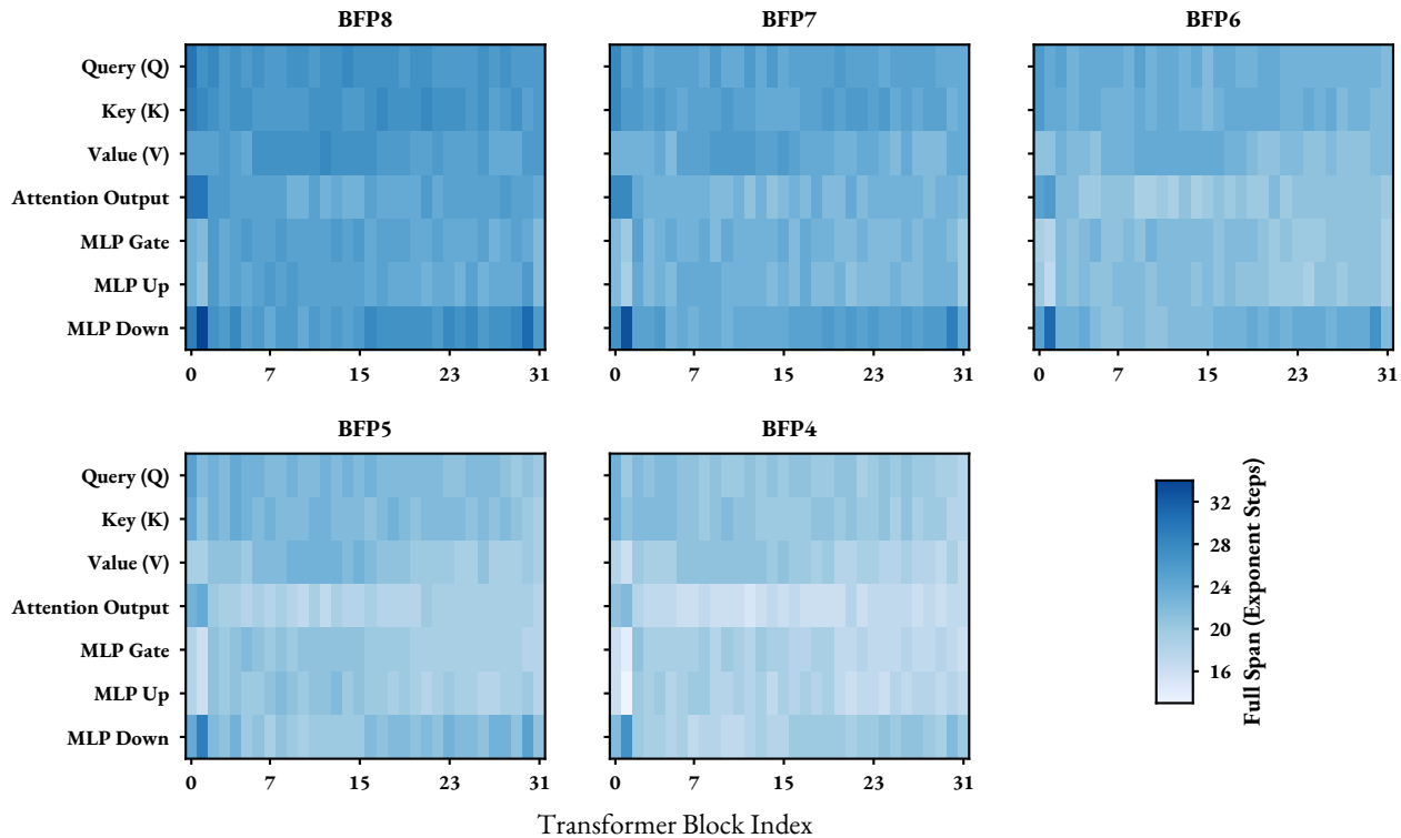
Per-Block Full Partial-sum Exponent Span
