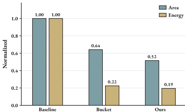
Figure 9: Normalized PE area and energy of a BFP4 baseline, a Bucket Getter PE, and the proposed PE (TSMC 90 nm, 125 MHz). Bucket Getter and the proposed PE count half of the FP-Acc area to model two-PE sharing. Both metrics are normalized to the baseline.
