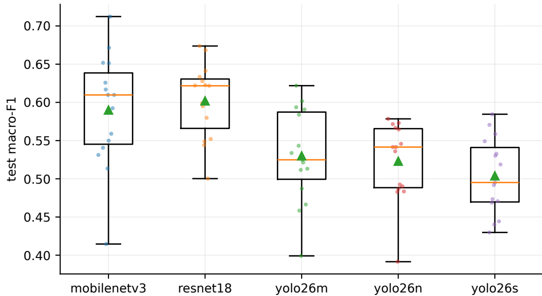
Cross-validated macro-F1 by architecture (5x3 folds)
