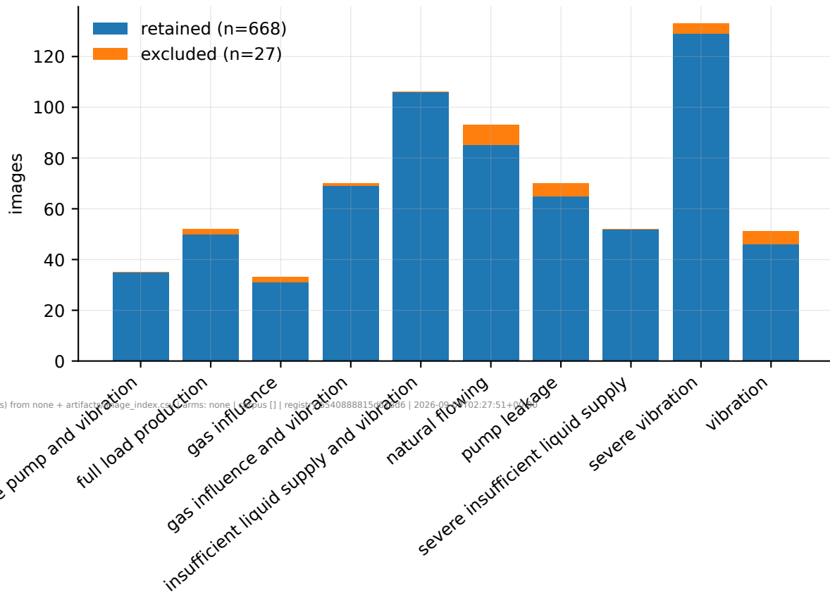
Class distribution before and after duplicate-label exclusion
