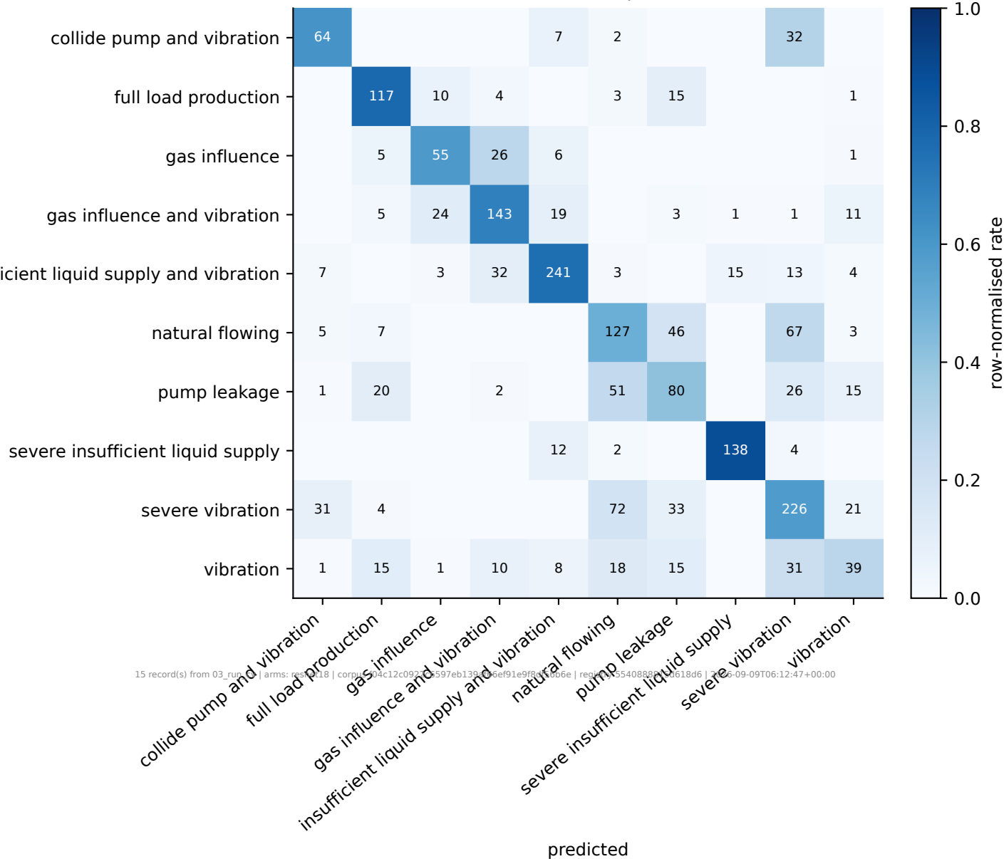
Confusion matrix, resnet18 (frontier) -- 2004 predictions summed over all 15 folds
