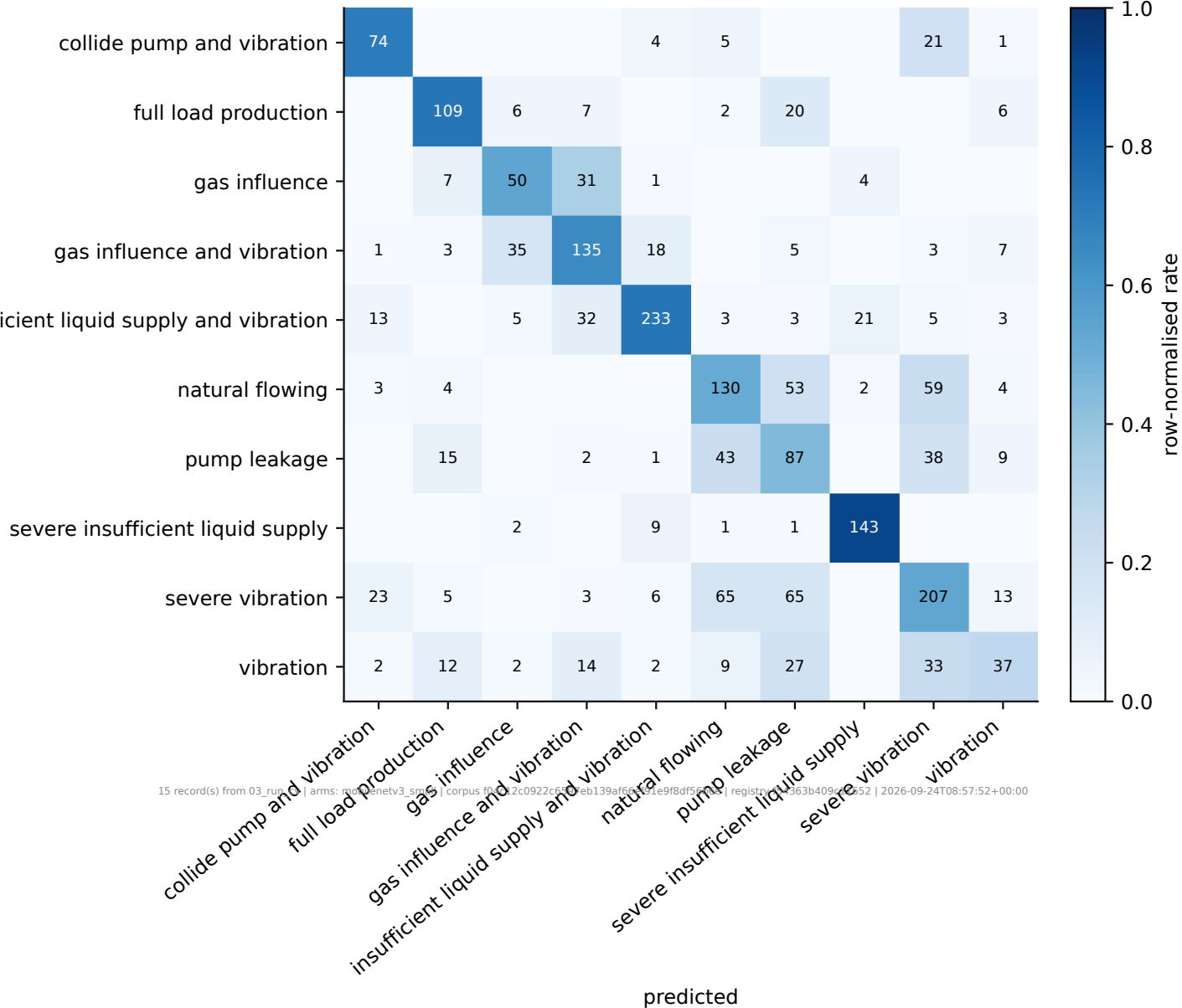
Confusion matrix, mobilenetv3_small (detailed) -- 2004 predictions summed over all 15 folds
