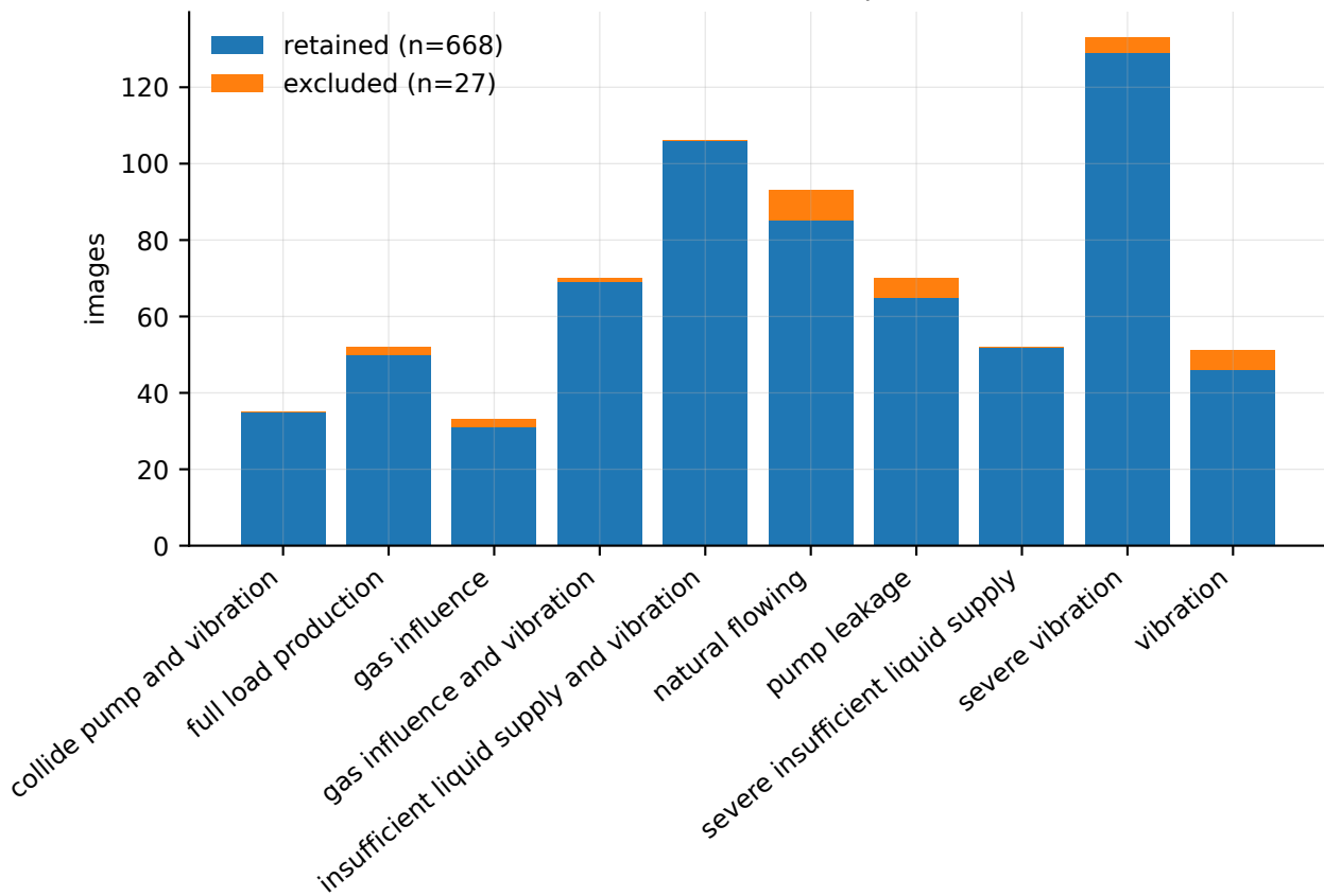
Class distribution before and after duplicate-label exclusion
