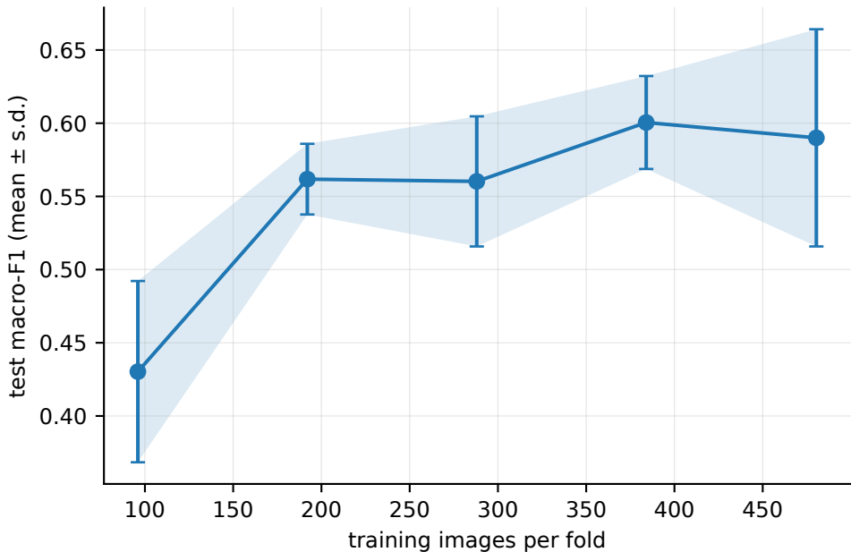
Learning curve under the locked mobilenetv3_small configuration
