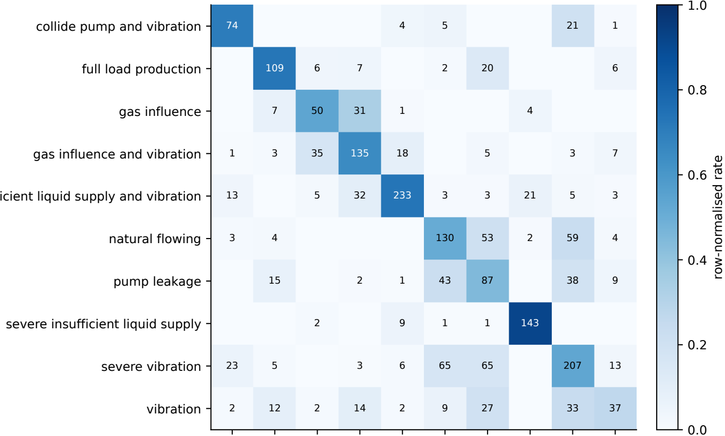
Confusion matrix, mobilenetv3_small (detailed) -- 2004 predictions summed over all 15 folds
